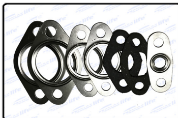
Part No : ATL AP I-27 Description : SILENCER PKG SET BS3 Suitable For : APE MRP : 56
