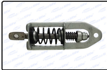
Part No : ATL AP F-10 Description : GOVERNOR SPRING ASSY Suitable For : APE MRP : 46
