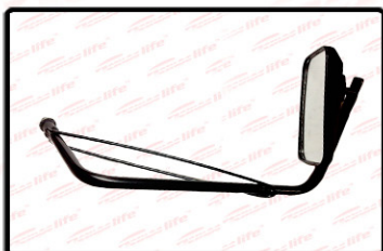
Part No : TLAP T-04 Description : OUTER REAR VIEW MIRROR LH ASSY Suitable For : APE MRP : 250
