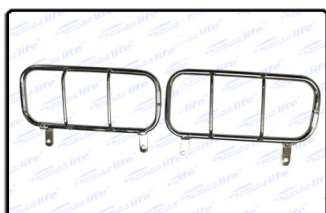
Part No : ATL AP Z-37 Description : TAIL LIGHT SHOW GUARD STEEL Suitable For : APE MRP : 270
